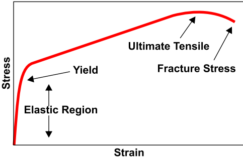
Stress - Strain Curve for Typical Tensile Test
